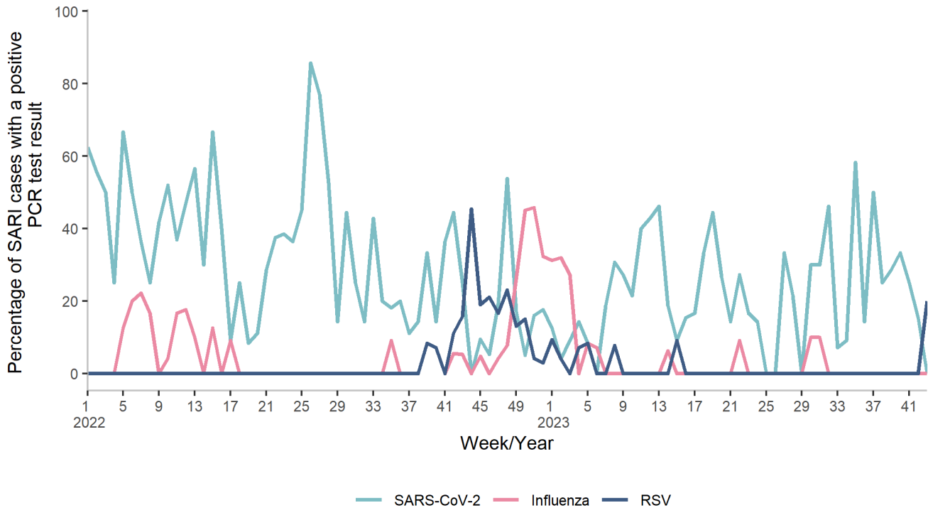
Figure 3 Percentage of SARI cases with a positive laboratory test result for SARS-CoV-2, influenza and RSV by week, from week 1 2022 to week 43 2023.
